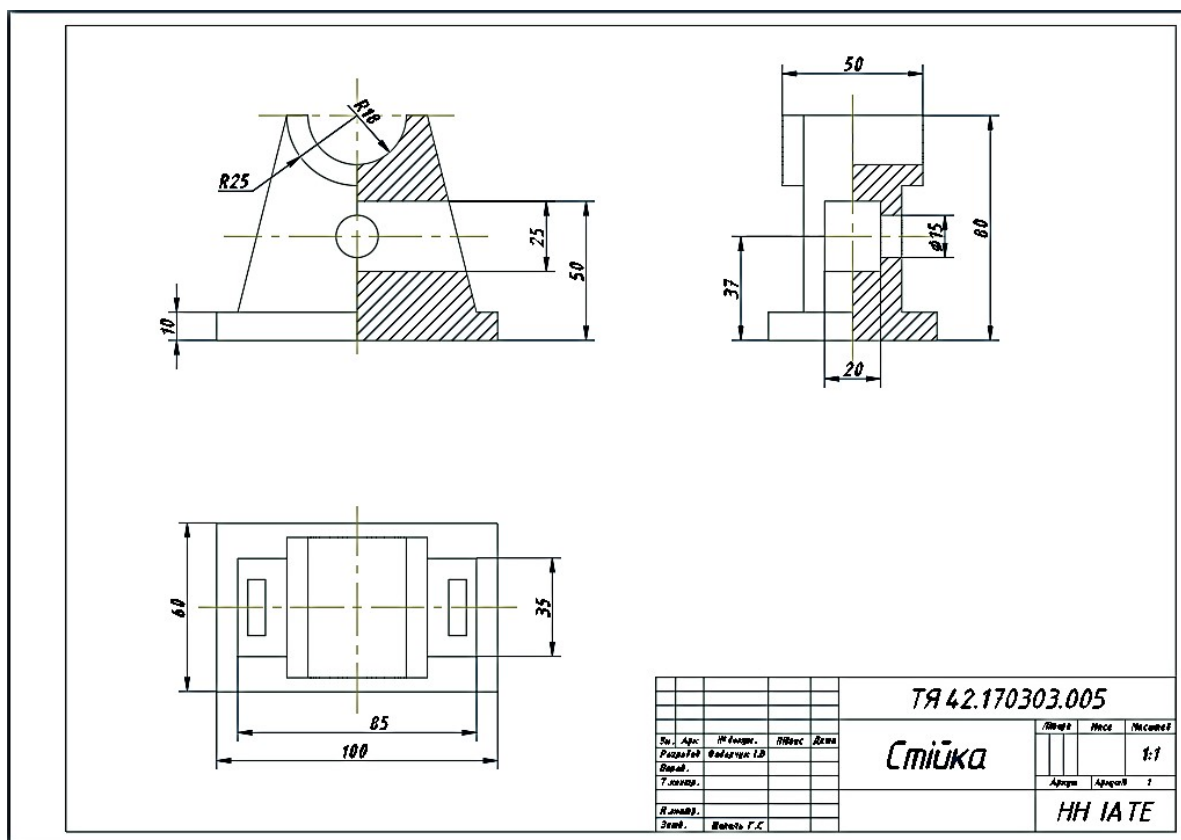
Fig. 2. Projection drawing generated from the solid model in Fig. 1
