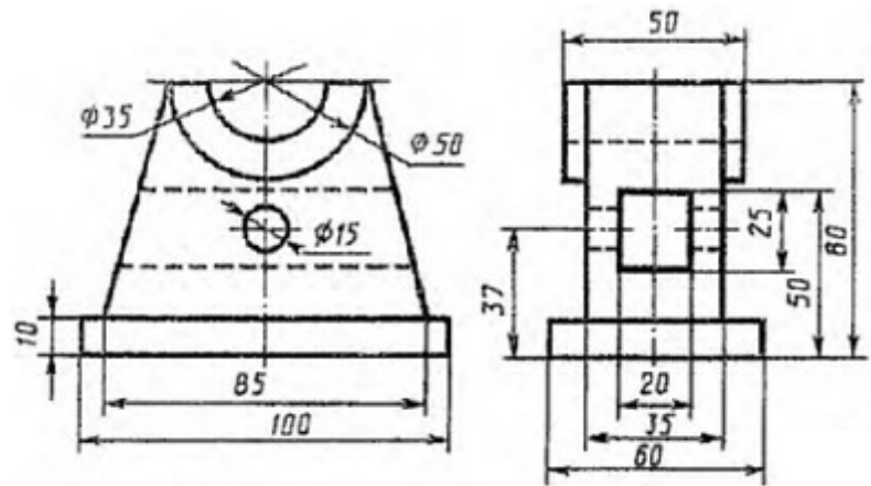
Fig. 1. Solid model and initial task for the laboratory assignment
